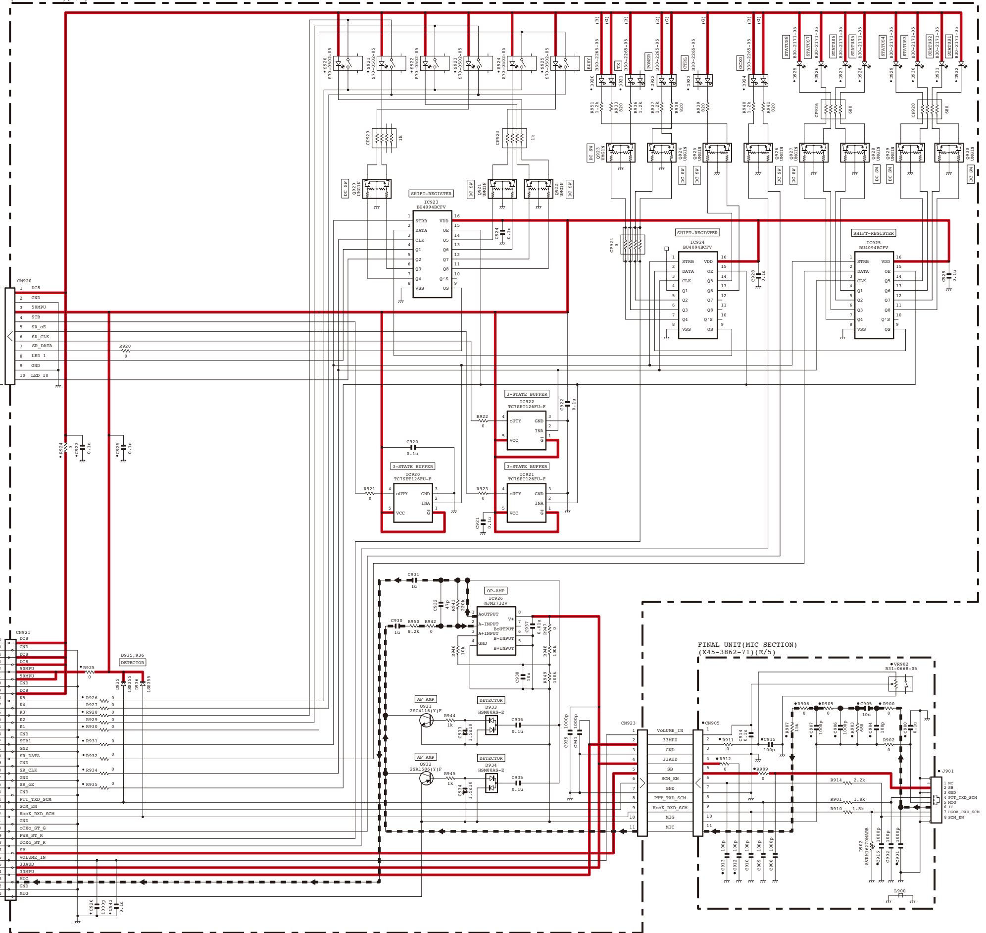
TX UNIT (LED) (X56-3120-12) (B/3)
