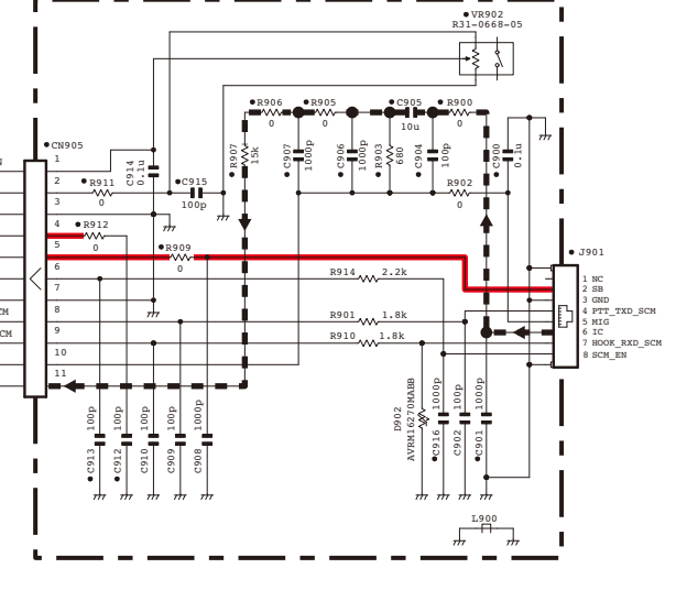
FINAL UNIT (MIC SECTION) (X45-3862-71) (E/5)
