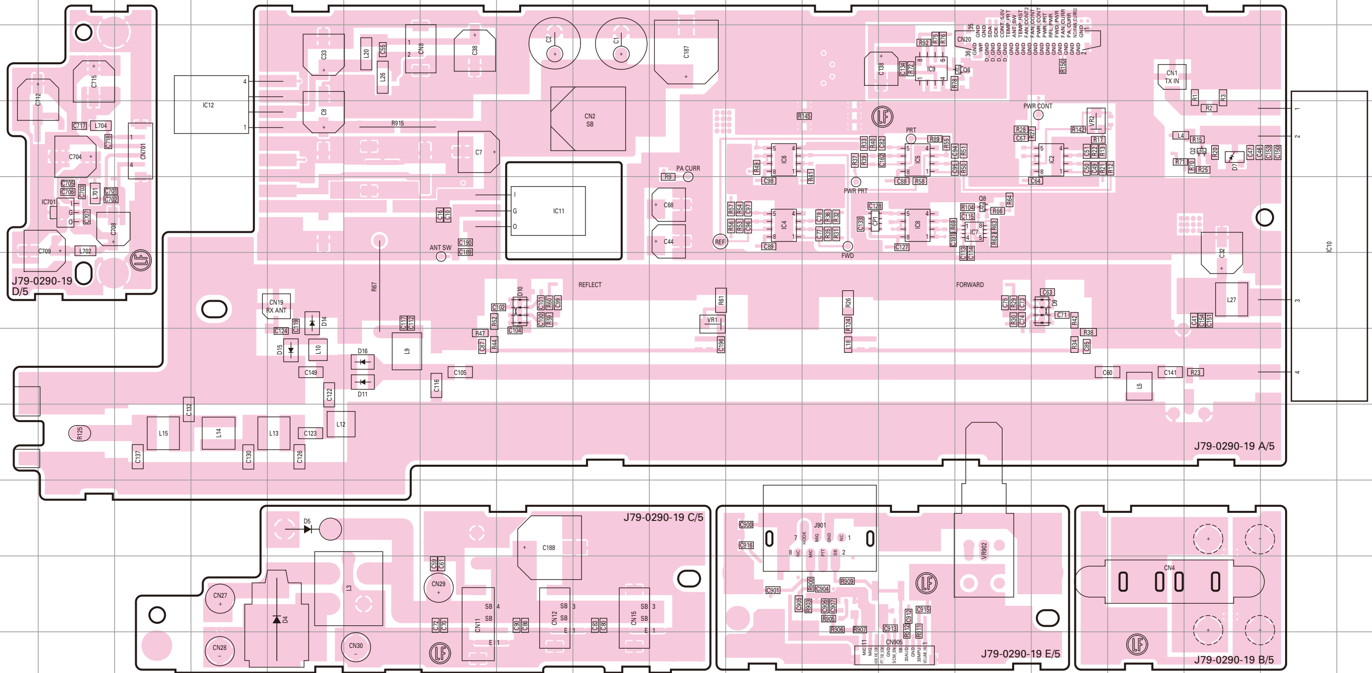
FINAL UNIT (X45-3862-71) Component side view (J79-0290-19)
